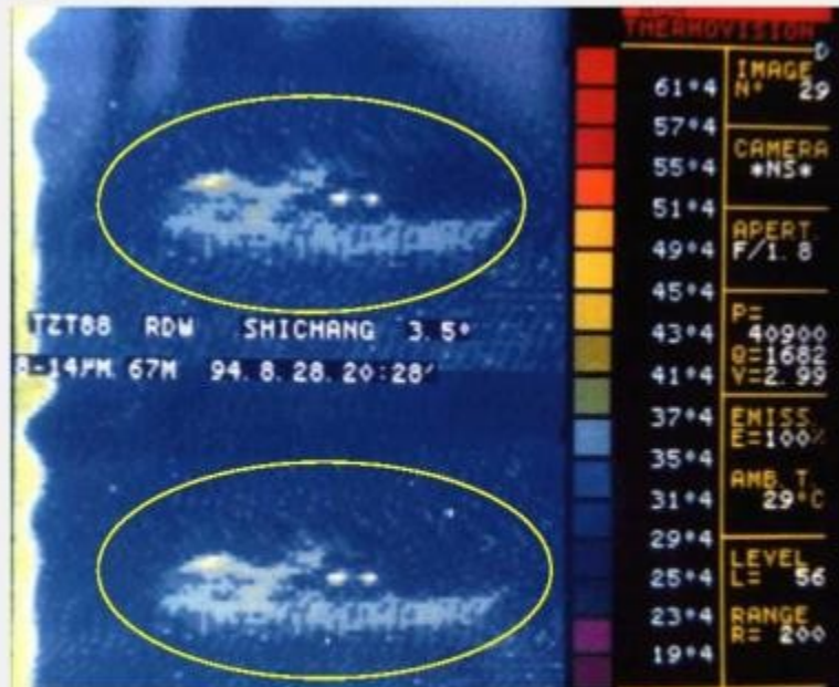
Infrared image : Tank is camouflaged by anti-infrared camouflage net
